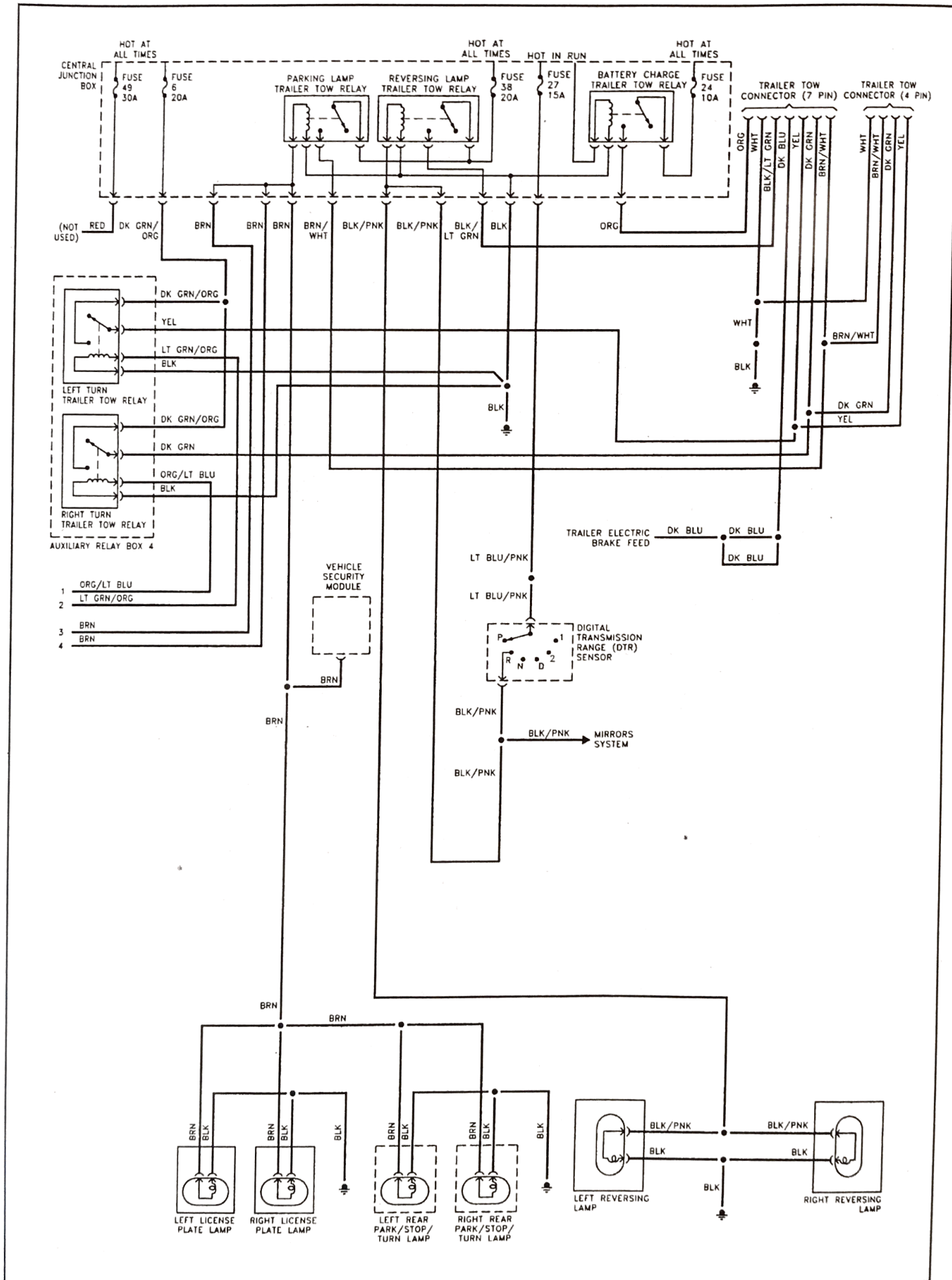
Exterior lighting system (except headlights) - 2002 and later Excursion models (2 of 2)
